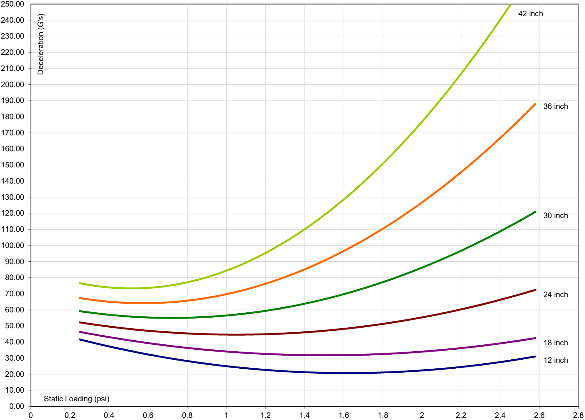
PolyPlank EXT 2.2pcf 2 x 48 Dynamic Cushion Curves AVE Drops 2-5 G @ Indicated Drop Height
