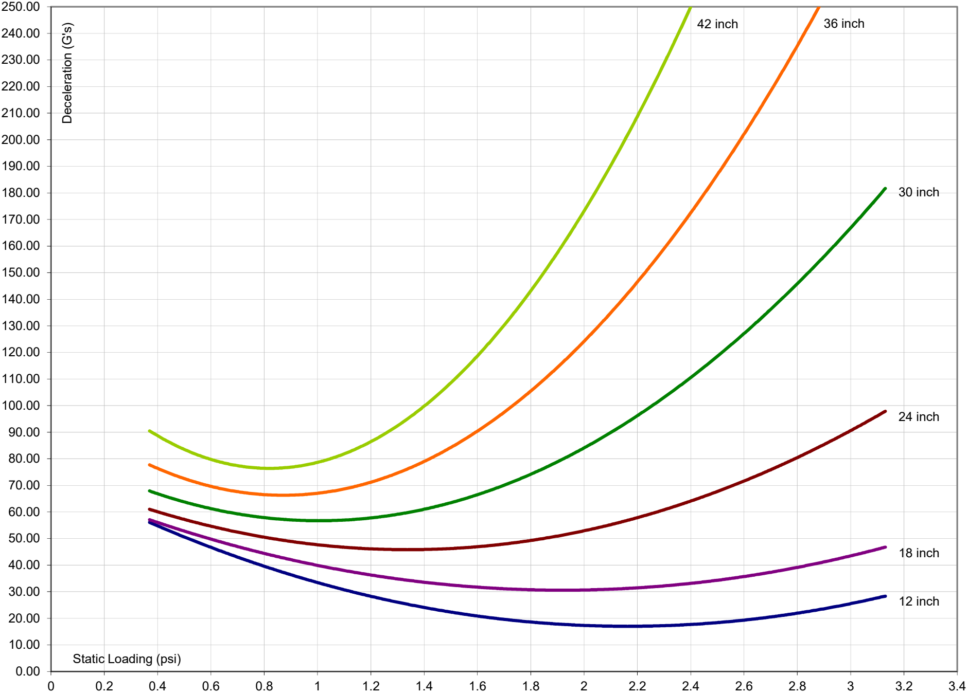
PolyPlank EXT 4.0pcf 2 x 24 Dynamic Cushion Curves AVE Drops 2-5 G @ Indicated Drop Height
