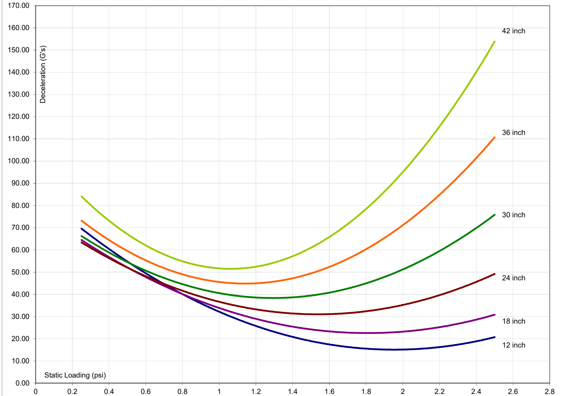
PolyPlank EXT 4.0pcf 2 x 24 Dynamic Cushion Curves Drop 1 G @ Indicated Drop Height
