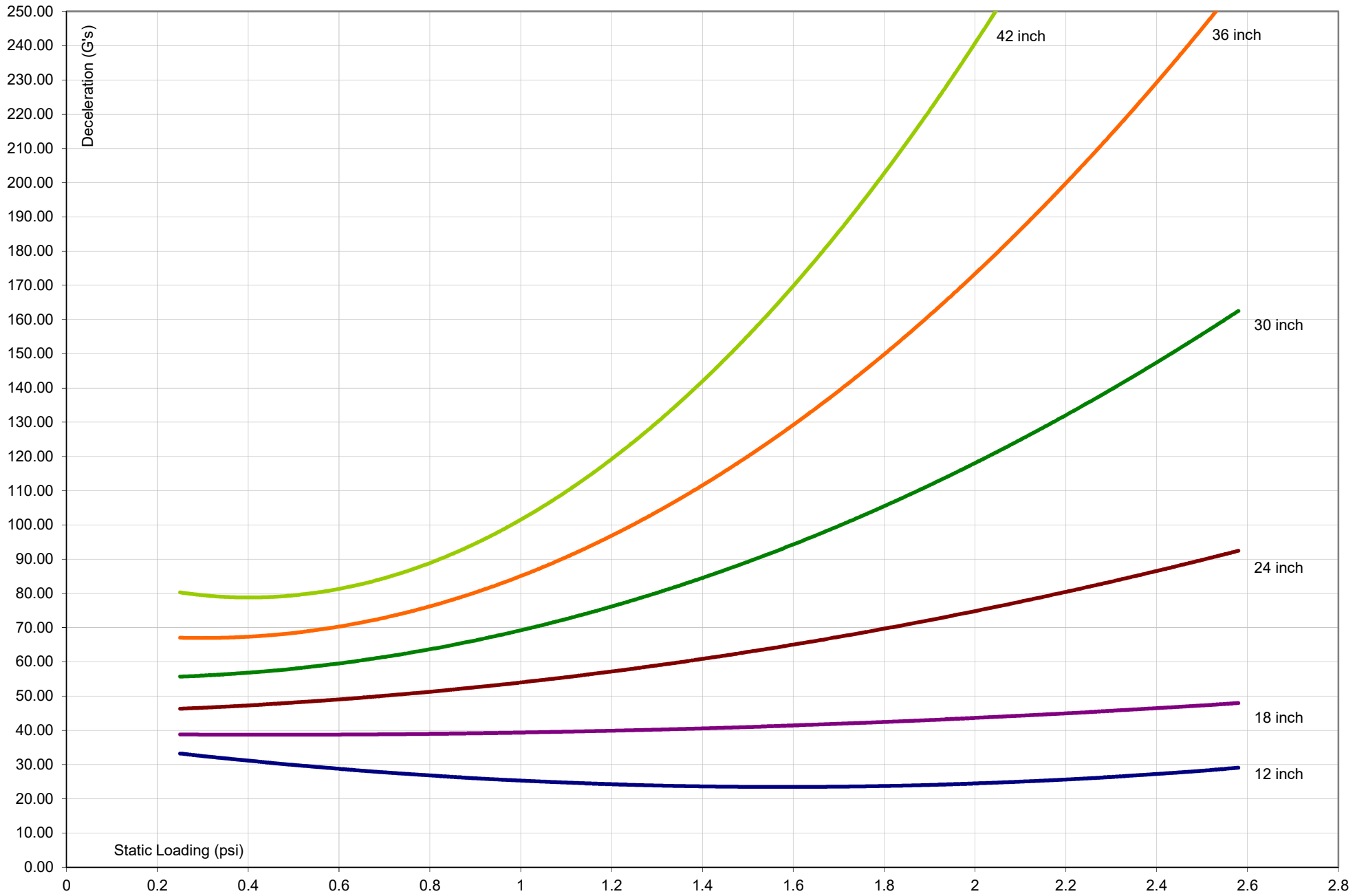
PolyPlank LAM 1.7pcf 2 x 48 LAM Dynamic Cushion Curves AVE Drops 2-5 G @ Indicated Drop Height
