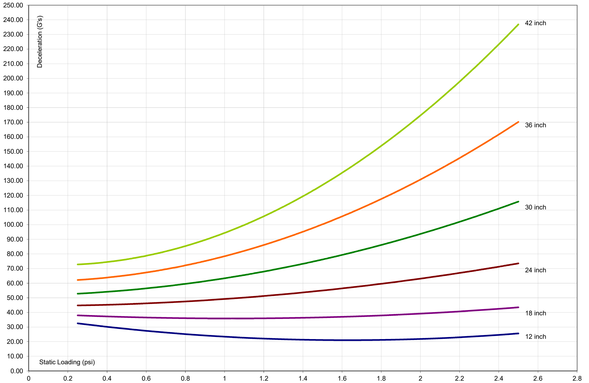
PolyPlank LAM 1.7pcf 2 x 48 Dynamic Cushion Curves Drop 1 G @ Indicated Drop Height
