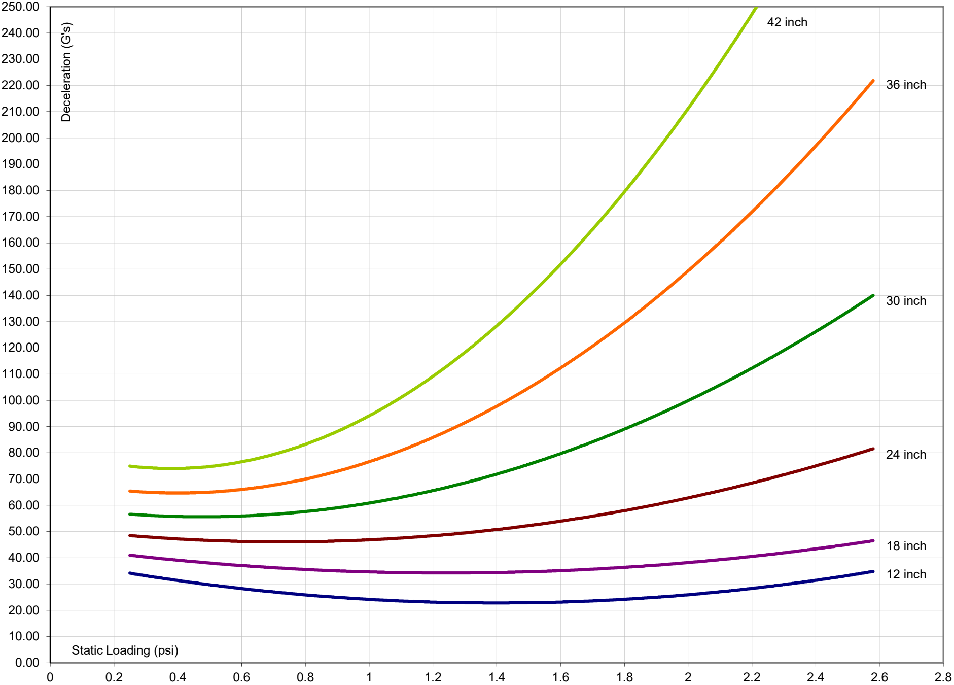
PolyPlank LAM 2.2pcf 2 x 48 Dynamic Cushion Curves AVE Drops 2-5 G @ Indicated Drop Height
