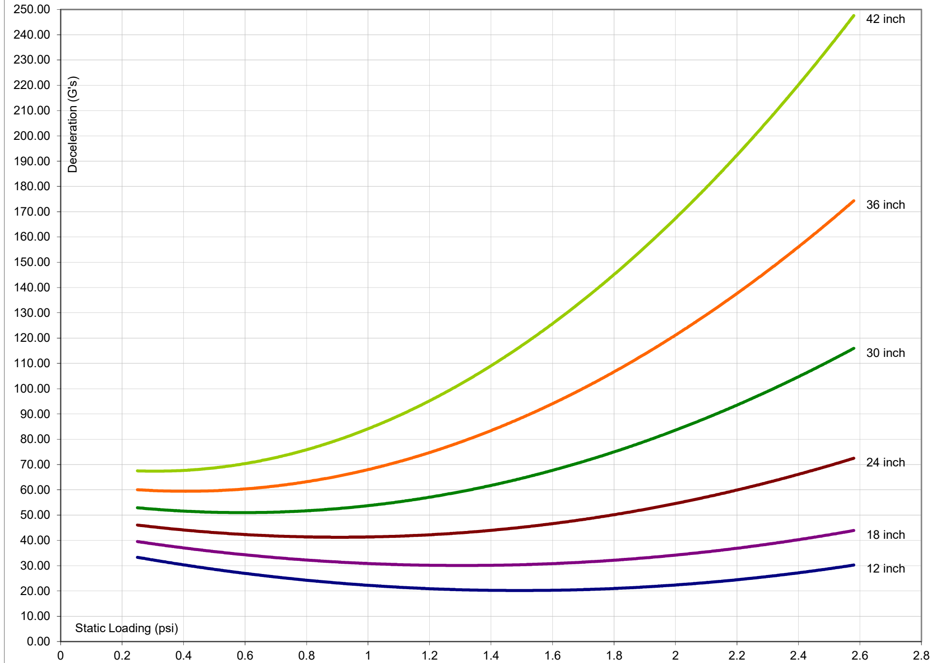
PolyPlank LAM 2.2pcf 2 x 48 Dynamic Cushion Curves Drop 1 G @ Indicated Drop Height
